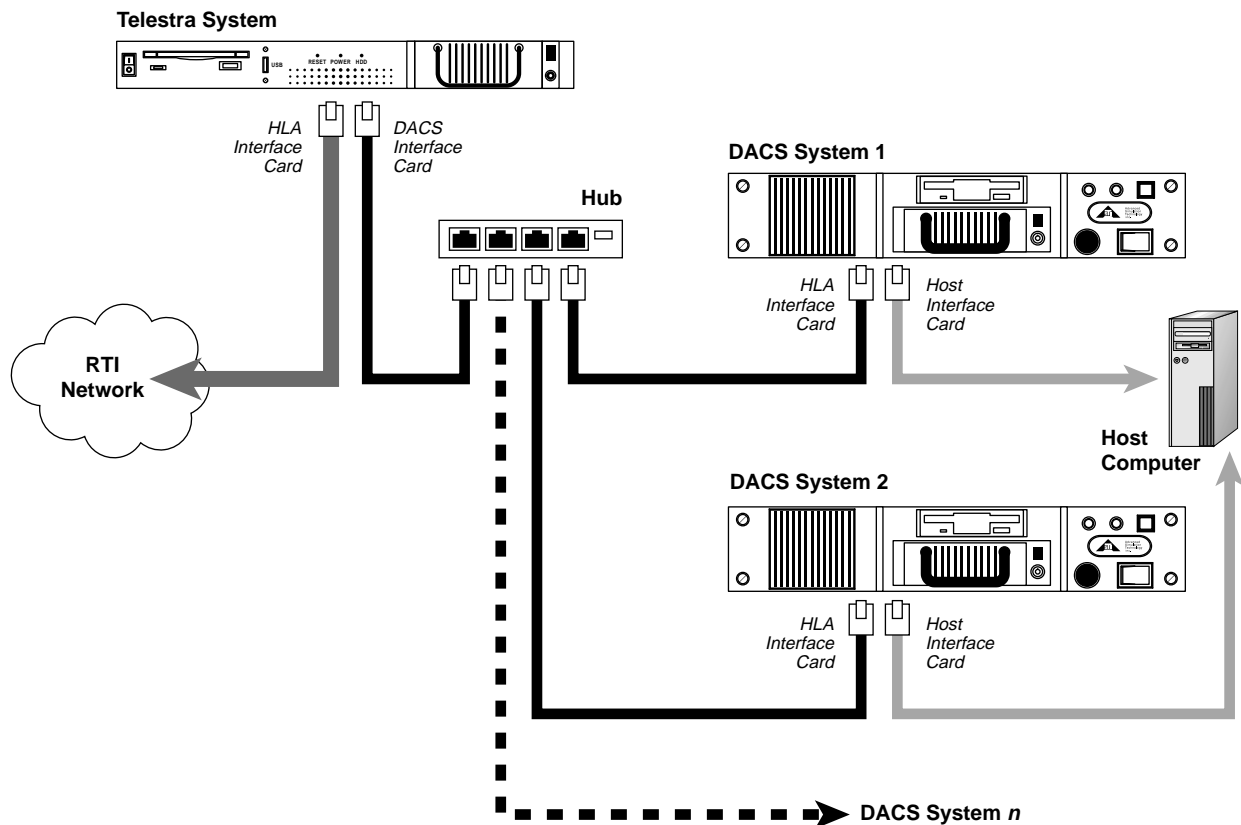
Figure 1: Correct wiring setup for the Telestra system.
