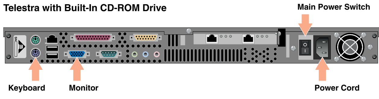
Figure 1: Telestra Connections Diagram
