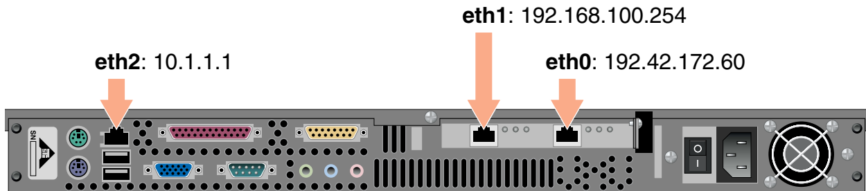
Figure 2: Ethernet Interface Locations & Default IP Addresses
